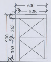
WORKING TABLE DETAIL (WOODEN DETAIL) DETAIL AT A SCALE: 1:20
