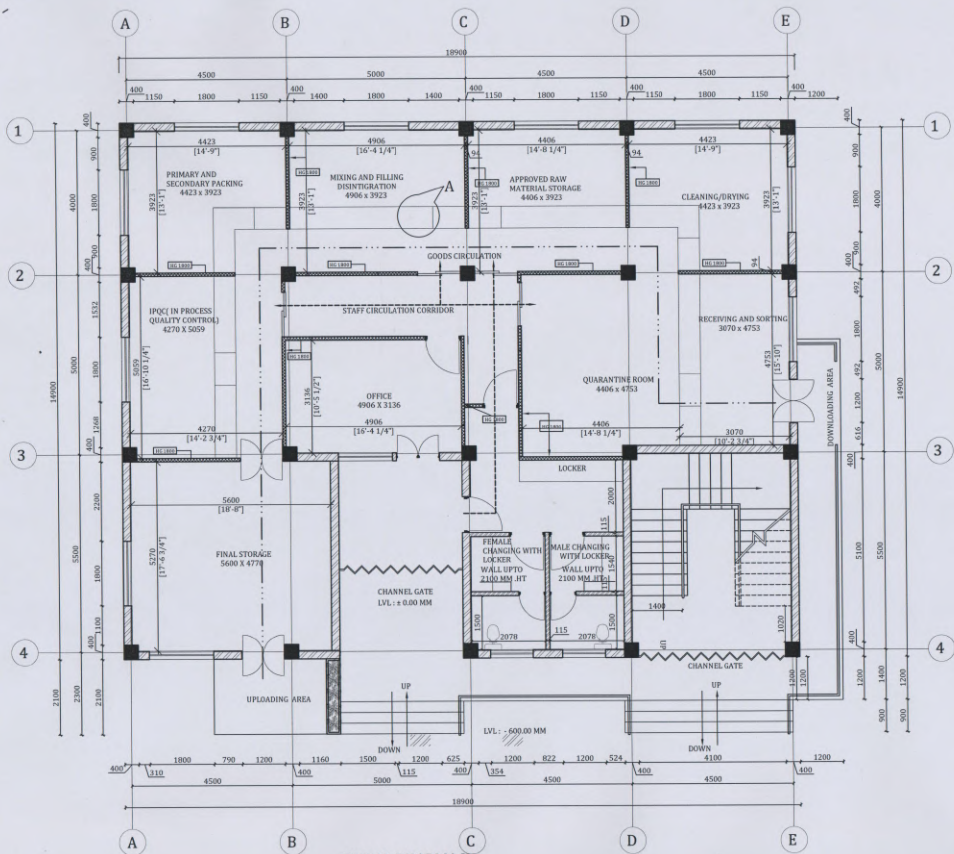
RURAL PHARMACY GROUND FLOOR PLAN (281.61 SQ. M.)
