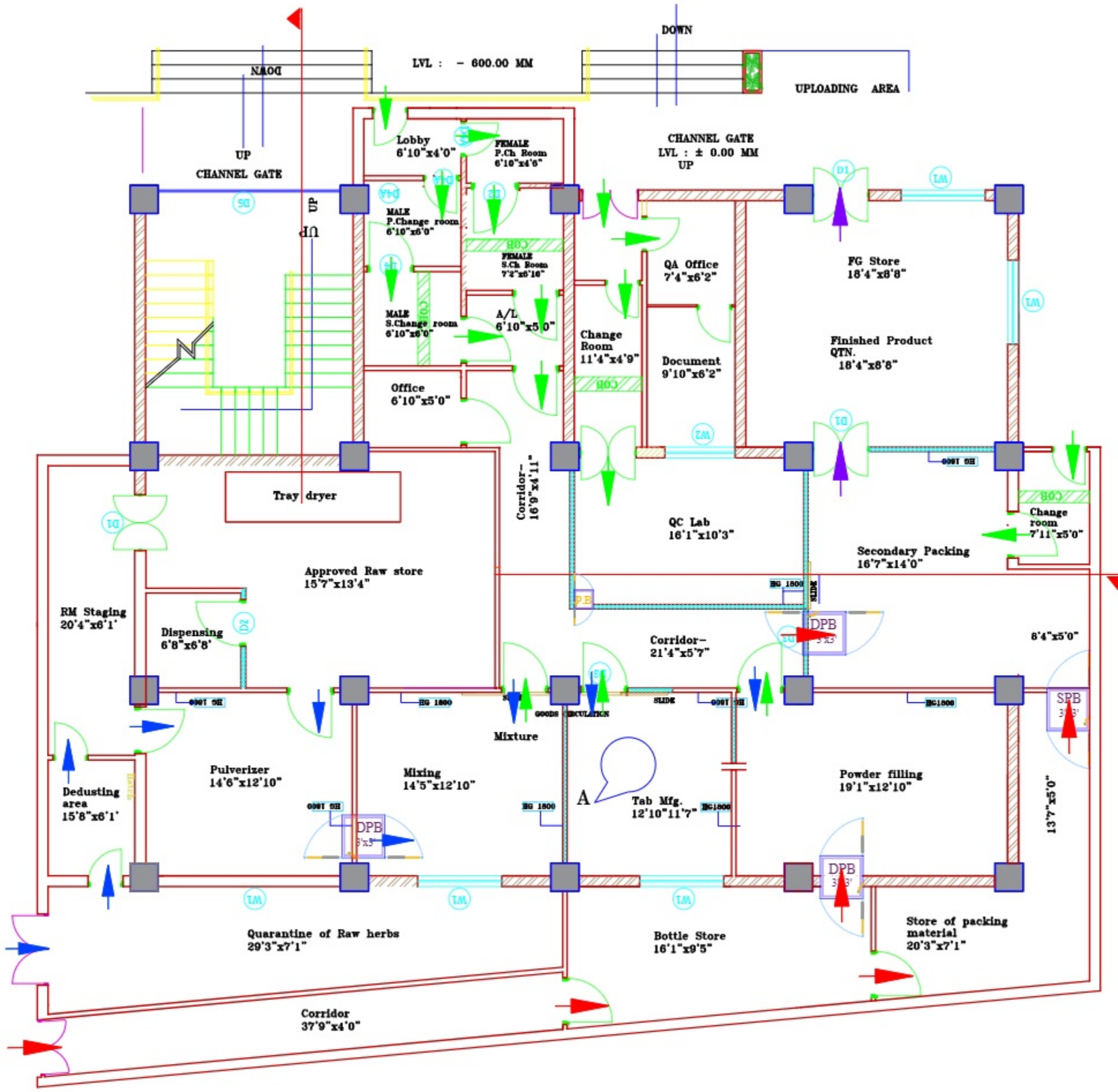
AYURVEDA AUSHADHI UTPADAN KENDRA GROUND FLOOR PLAN (281.61 SQ. M.)
